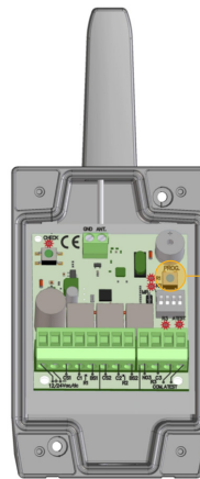
Receiver
