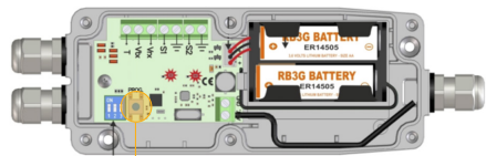
Transmitter
